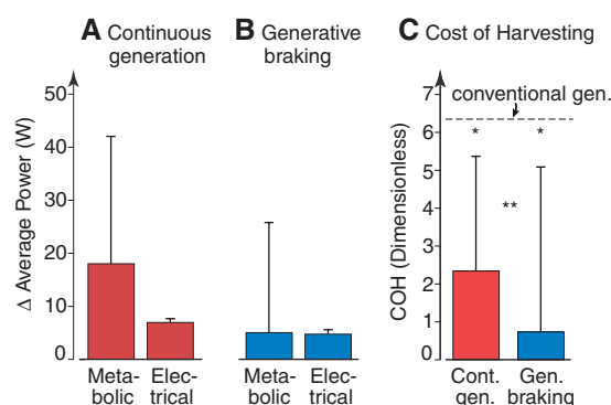
Fig. 4. Average metabolic cost and generated electricity for continuous generation (A) and generative braking (B), with change in metabolic cost ( \Delta average power) shown relative to the control condition. (C) COH (see Fig. 1) for continuous generation and generative braking as compared against that for conventional generation (dashed line). In both modes, a fraction of the harvested energy is generated from the deceleration of the knee rather than directly from muscle action. Error bars in (A) to (C) indicate SD. Asterisks indicate significant differences with conventional generation (*) and between continuous generation and generative braking (**) ( P < 0.05 for all comparisons).
