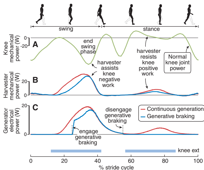
Fig. 3. Timing of power generation during walking.
