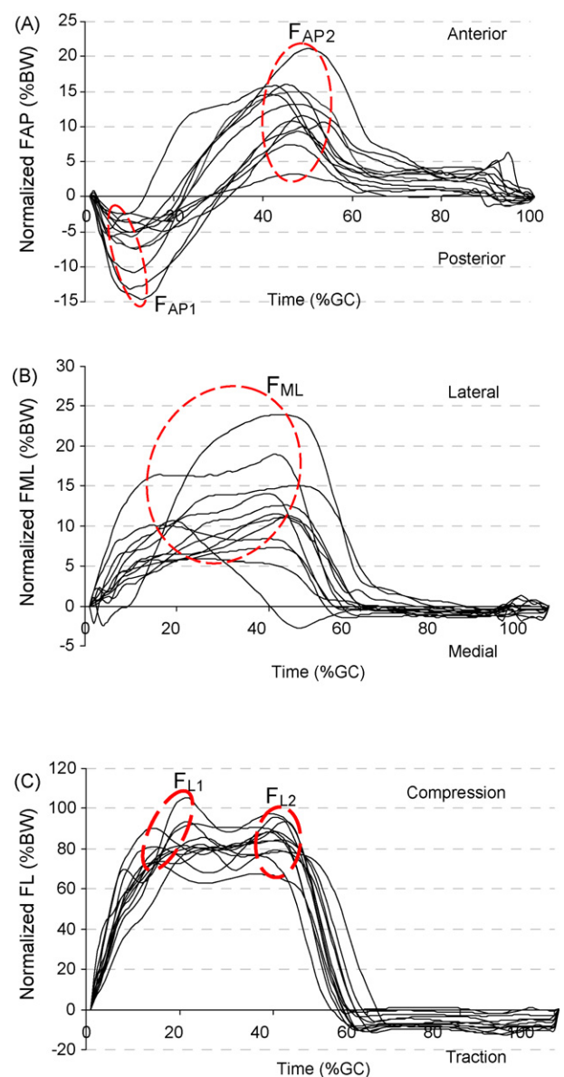
Fig. 3. Mean force expressed as a percentage of body weight of each subject applied on the abutment in (A) antero-posterior, (B) medio-lateral, and (C) long-axis directions for the 12 amputees versus percentage of gait cycle.
