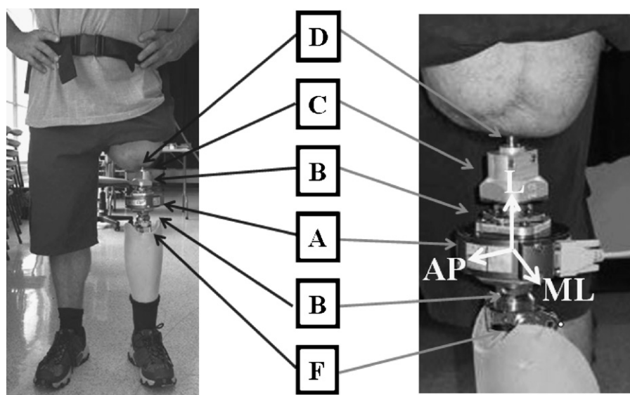
Fig. 2. Example of a typical prosthetic leg setup used to directly measure the forces and moments applied on the abutment of a transfemoral amputee (left: front view, right: side view). A commercial transducer (A) was mounted to specially designed plates (B) that were positioned between the adaptor (C) connected to the abutment (D) and the knee mechanism (F).
