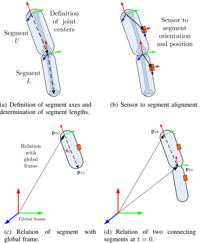
Fig. 4. Calibration and segment kinematics step.
